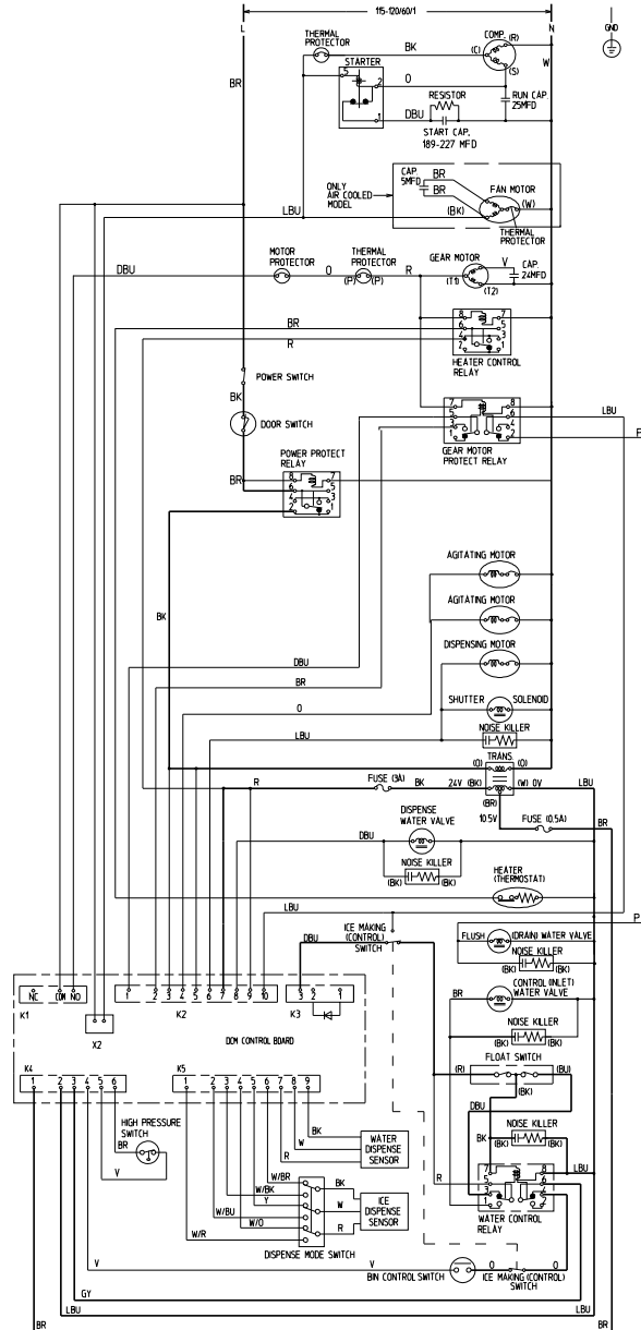
WIRE COLOR CODE
